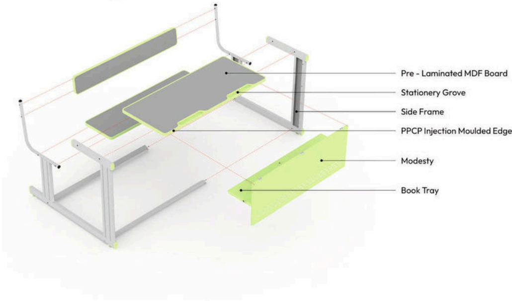
Flat Packaging
